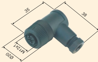
CCP12-4FA-G
