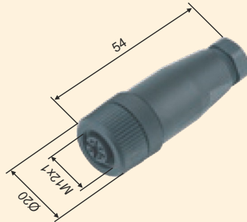
CCP12-4FS-G
